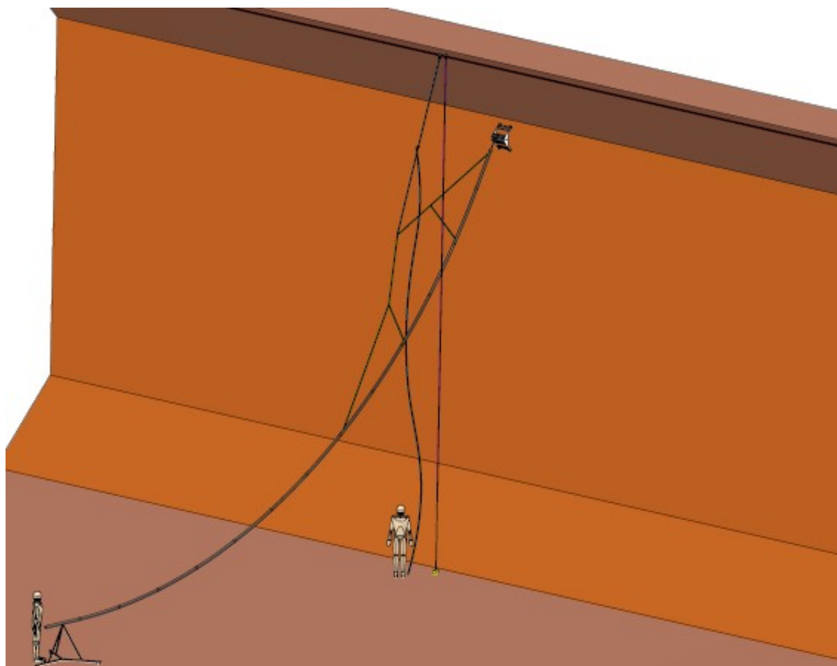
Illustration of the guide wire being used to lift the HR/HP Kit
